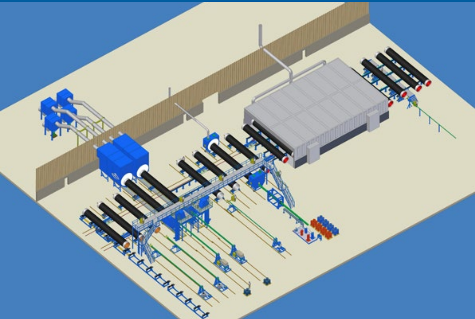
Internal blasting and coating plant
